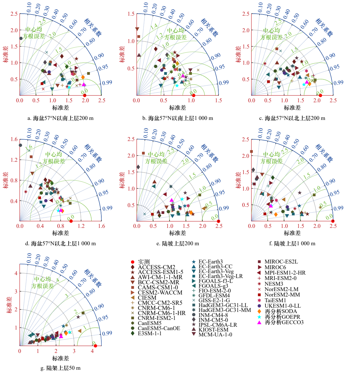
图6 2014年7月海盆、陆坡和陆架区海温的空间泰勒图: CMIP6模式数据、再分析数据与实测数据比较 Fig. 6 Taylor diagrams of sea temperature in July 2014 for the basin, continental slope and shelf: comparison between CMIP6 model data, reanalysis data, and observational data
