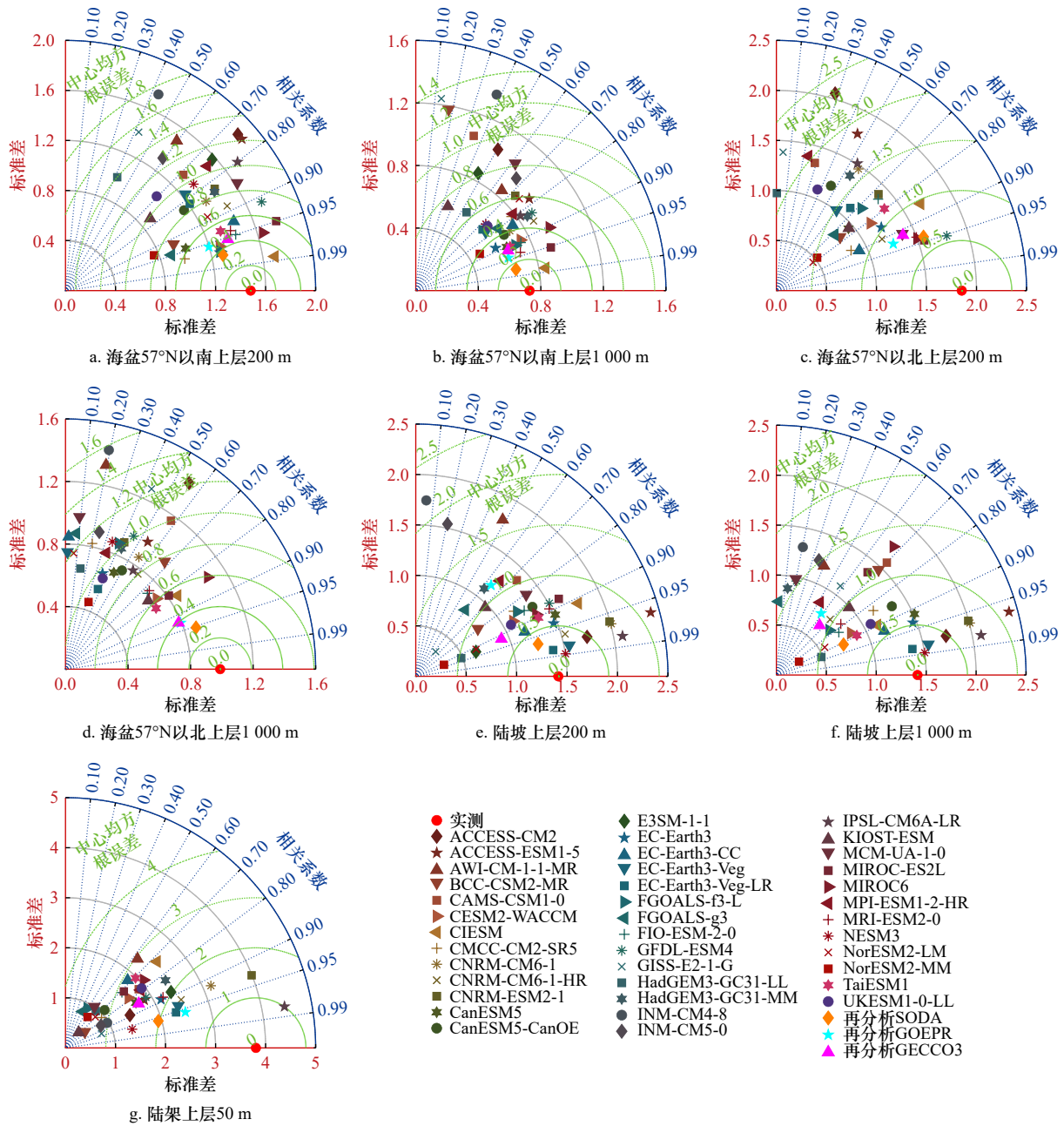
图5 2012年7月海盆、陆坡和陆架区海温的空间泰勒图: CMIP6模式数据、再分析数据与实测数据比较 Fig. 5 Taylor diagrams of sea temperature in July 2012 for the basin, continental slope and shelf: comparison between CMIP6 model data, reanalysis data, and observational data
