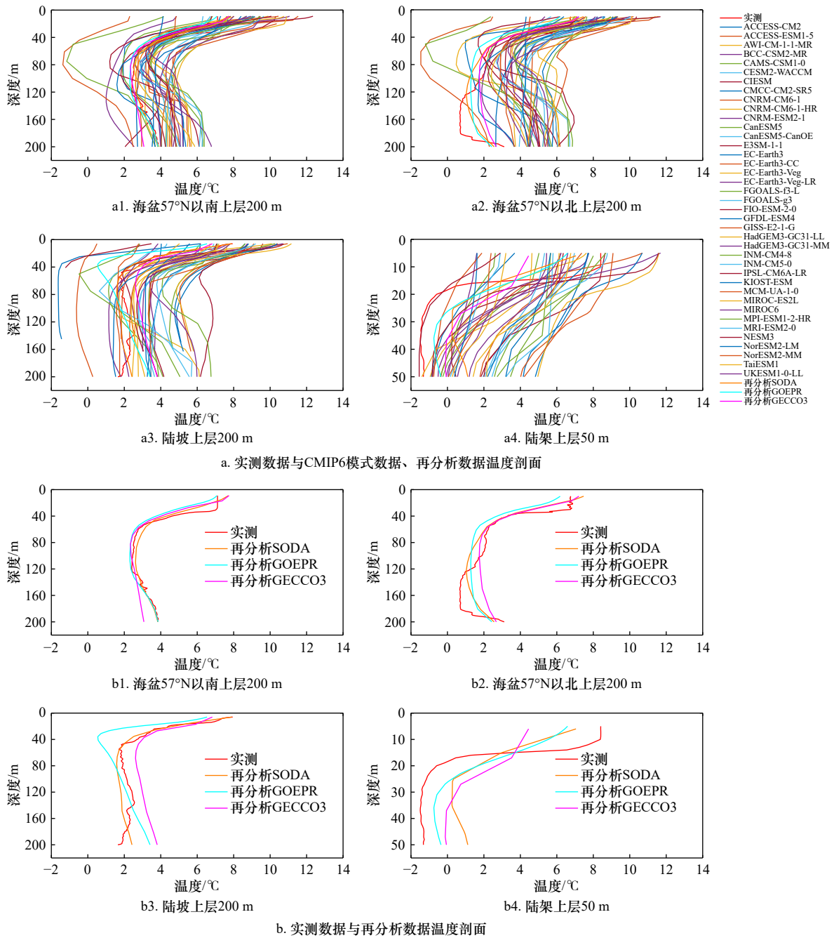
图1 2012年7月CMIP6模式数据、再分析数据与实测数据的海盆、陆坡和陆架上层200m以浅温度剖面 Fig. 1 Temperature profiles within the upper 200 m based on CMIP6 model data, reanalysis data, and observational data in July 2012 over the basin, continental slope and shelf
